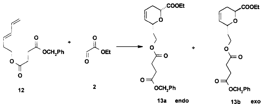
Scheme 3 Diels-Alder reaction by polyclonal antibody catalysis.
