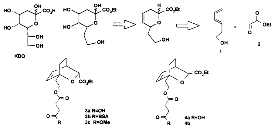
Scheme 1 Retrosynthetic analysis of KDO analog and the bridge compounds designed as the hapten and antigen.
